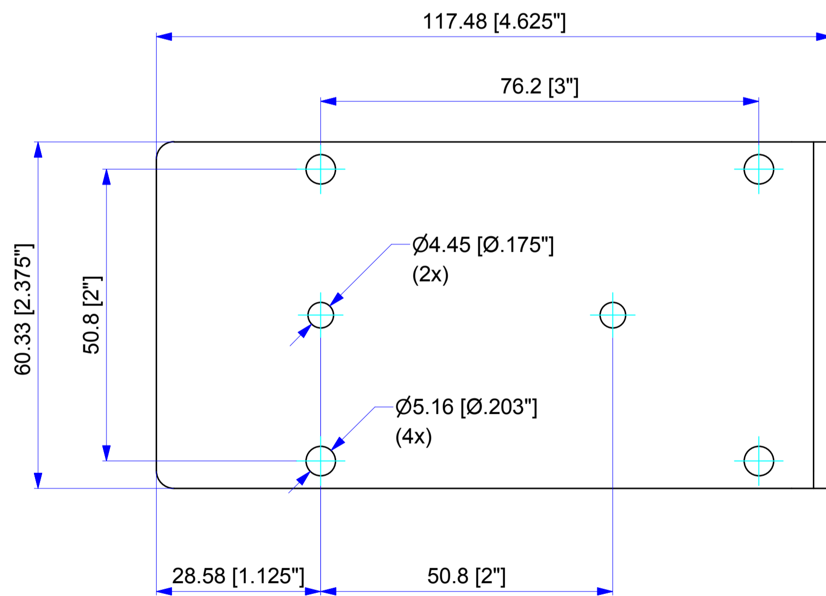
Dimension in mm [Inch]
