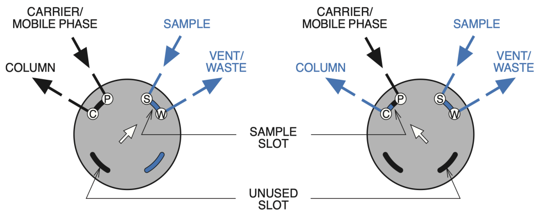
FIGURE 1: Valve viewed from the preload end
