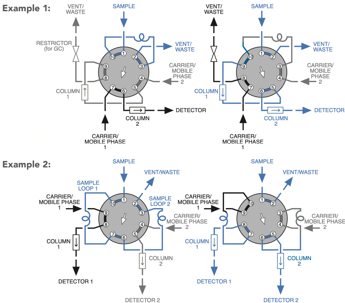
FIGURE 1: Valve viewed from the preload end
